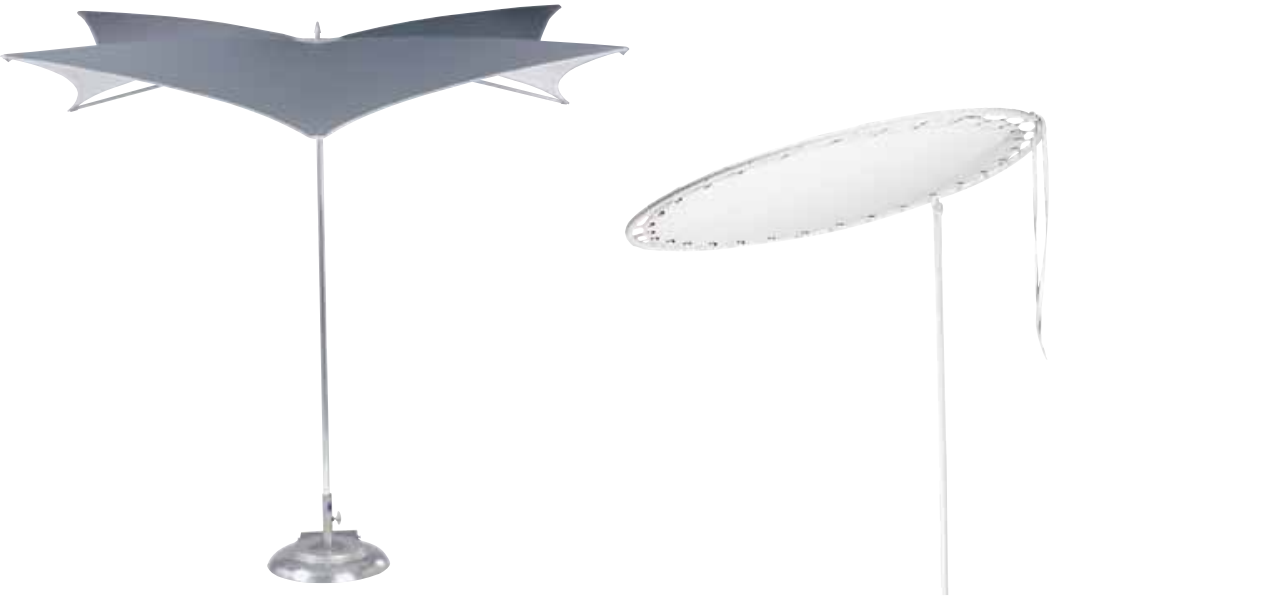
1390-9820 8-1/2' Square Manta™ / Auto-Loc-Pulley / 1-1/2" Anodized Aluminum, One Piece Pole 102w x 102l x 96h
